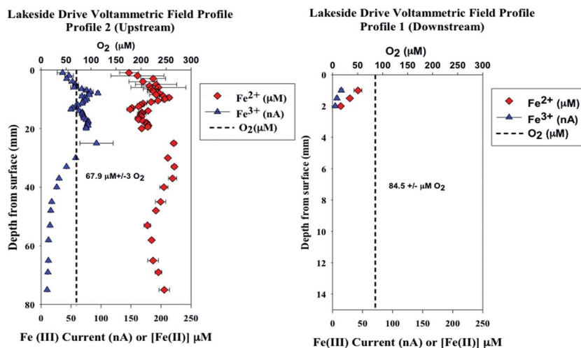
Fig. 4 Profiles of Fe(II), Fe(III) and \text{O}_2 from the upstream and downstream sampling sites from Lakeside Drive, ME.
