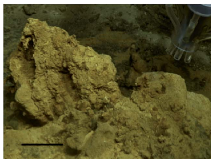
Fig. 2 Image of microbial mat (with the tip of the syringe sampler) near the Rainbow vent site. Marker bar = 5 cm.
