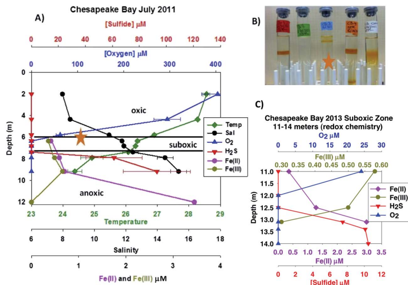
Fig. 1 (a) Representative vertical profile from the Chesapeake Bay in July of 2011 with sulfide, oxygen, Fe(II), Fe(III), temperature, and salinity plotted vs. depth with each chemical zone (oxic, suboxic, and anoxic) shown; (b) images of FeCl 2 gradient tube cultures. Three tubes show distinct, sharp orange bands, indicating positive FeOB growth from the Chesapeake Bay. The right-most tube is the uninoculated control, showing a diffuse orange band, indicating abiotic Fe(II) oxidation; (c) Fe(II), Fe(III), O 2 , and H 2 S concentrations found around the suboxic zone from the Chesapeake cruise in 2013.
