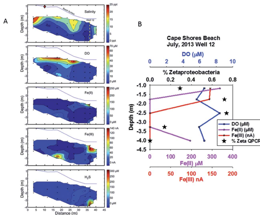
Fig. 3 (a) Contour plots showing changes in salinity, dissolved oxygen (DO), Fe(II), Fe(III), and \text{H}_2\text{S} with depth as well as distance from the benchmark in the dunes. Black dots represent well sampling depths, while the blue line indicates the beach surface, sloping towards the ocean. Well 12, shown in (b), is indicated with a dashed yellow line. (b) Well 12 profiles of DO, Fe(II), and Fe(III) from Cape Shores July 2013 with % Zetaproteobacteria versus well depth (below beach surface).
